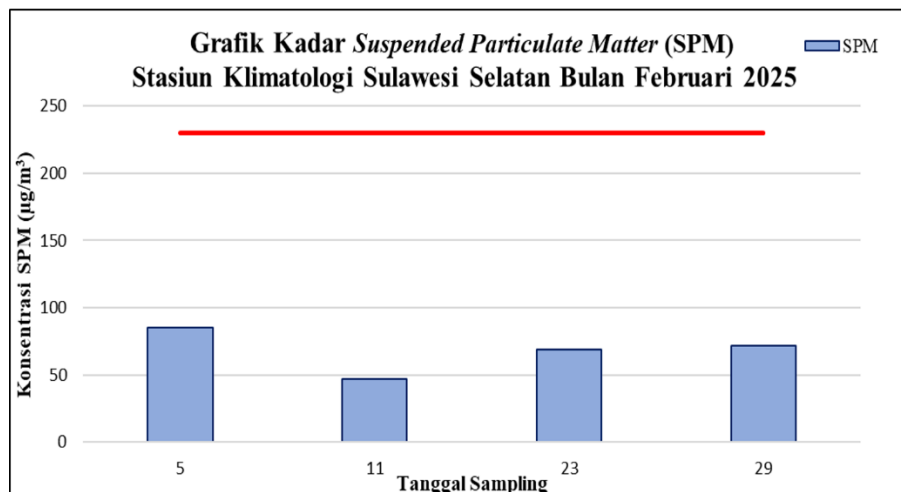
Gambar 24. Grafik Kadar Suspended Particulate Matter (SPM)
